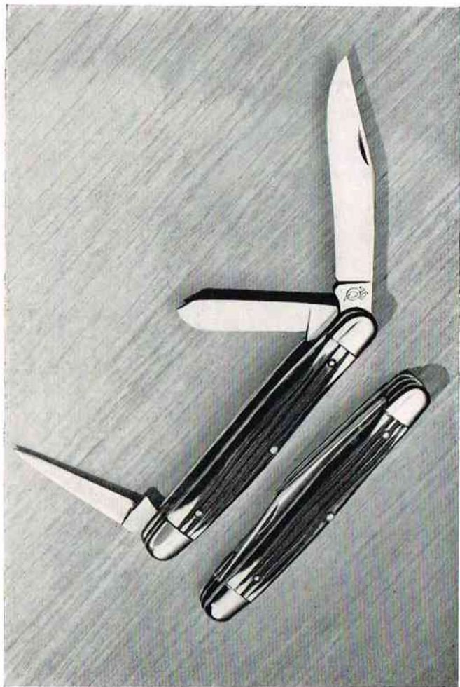
No. 37 Stockmen's Belt Punch Pattern — Large three blade knife. Genuine Frontier bone stag handle. Made of high carbon finest selected tool steel. Nickel Silver double bolsters, brass linings. One 2\frac{7}{8} -inch clip blade with 2\frac{5}{8} -inch cutting edge, one 1\frac{7}{8} -inch spey blade with 1\frac{5}{8} -inch cutting edge and one 1\frac{7}{8} -inch leather belt punch wire cutter blade with 1\frac{1}{8} -inch cutting edge. 4 inches long when closed.
